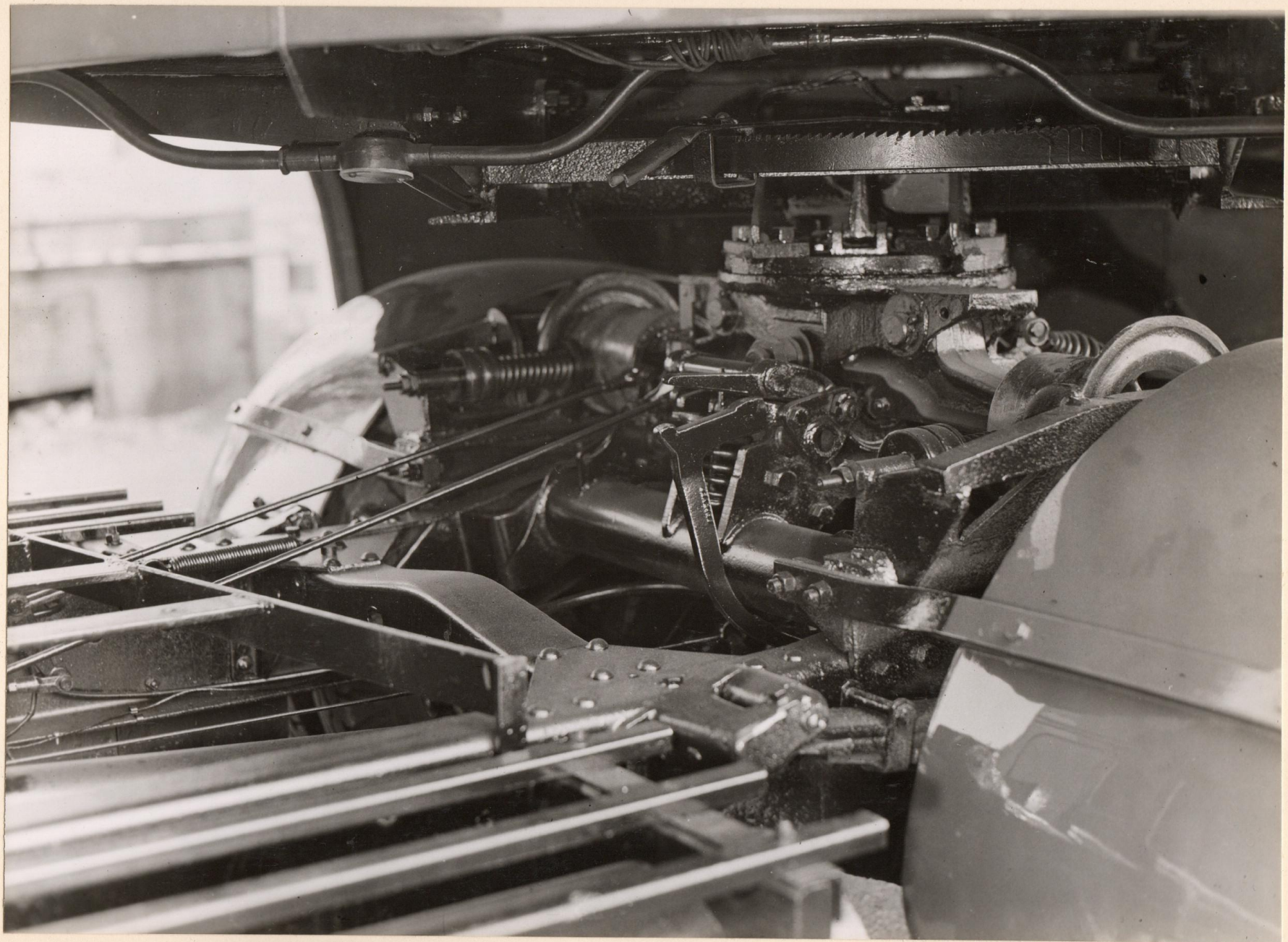
COUPLING GEAR BEDFORD - SCAMMELL - MOBILE CANTEEN 700 B.
