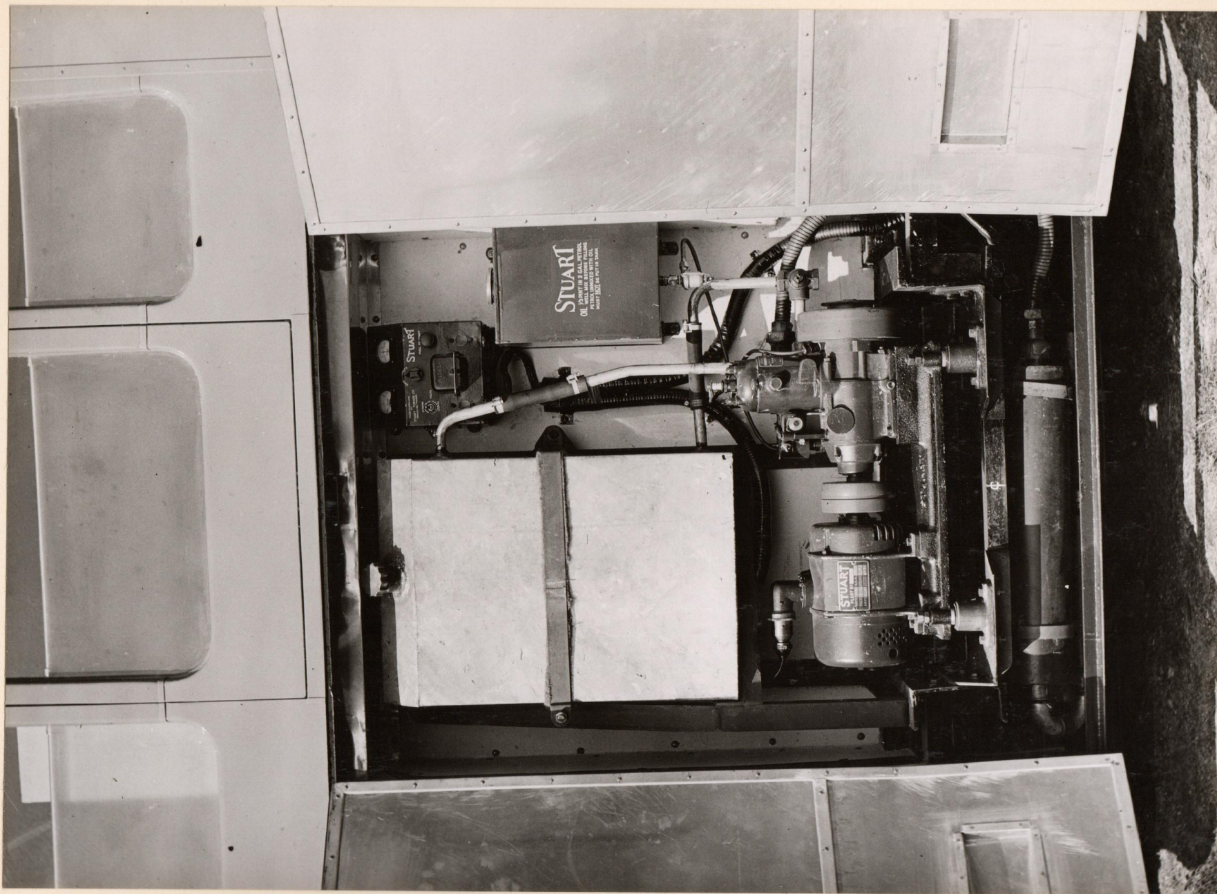
1 1/4 KW BATTERY CHARGING SET BEDFORD-SCAMMELL-MOBILE CANTEEN 700 B.
