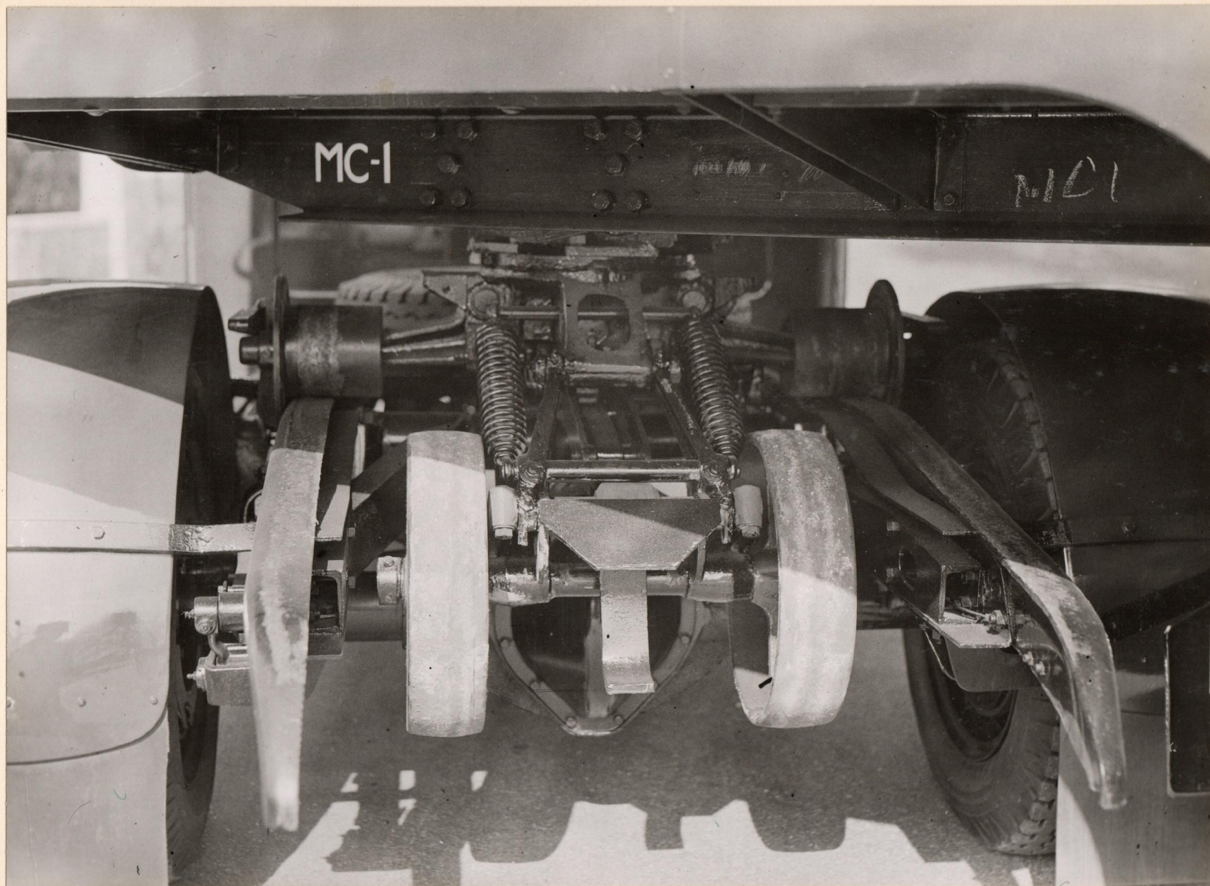
COUPLING GEAR BEDFORD-SCAMMELL -MOBILE CANTEEN 700 B.
