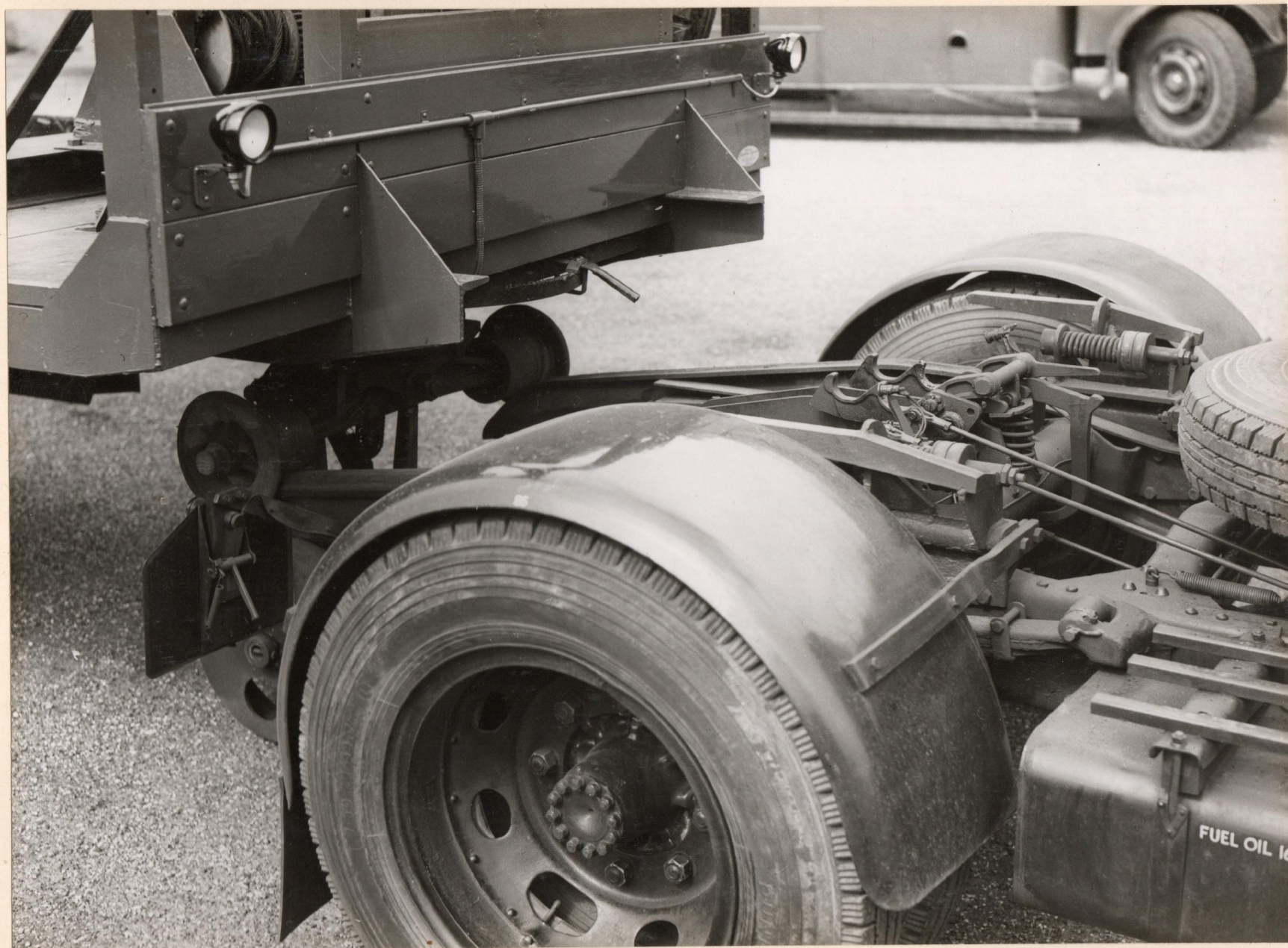
BEDFORD SCAMMEL COUPLING GEAR
