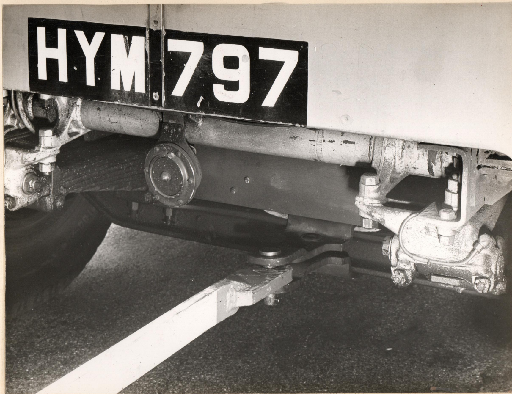
TROLLEYBUS SHEWING FRONT ATTACHMENT OF RIGID TOWING BAR
