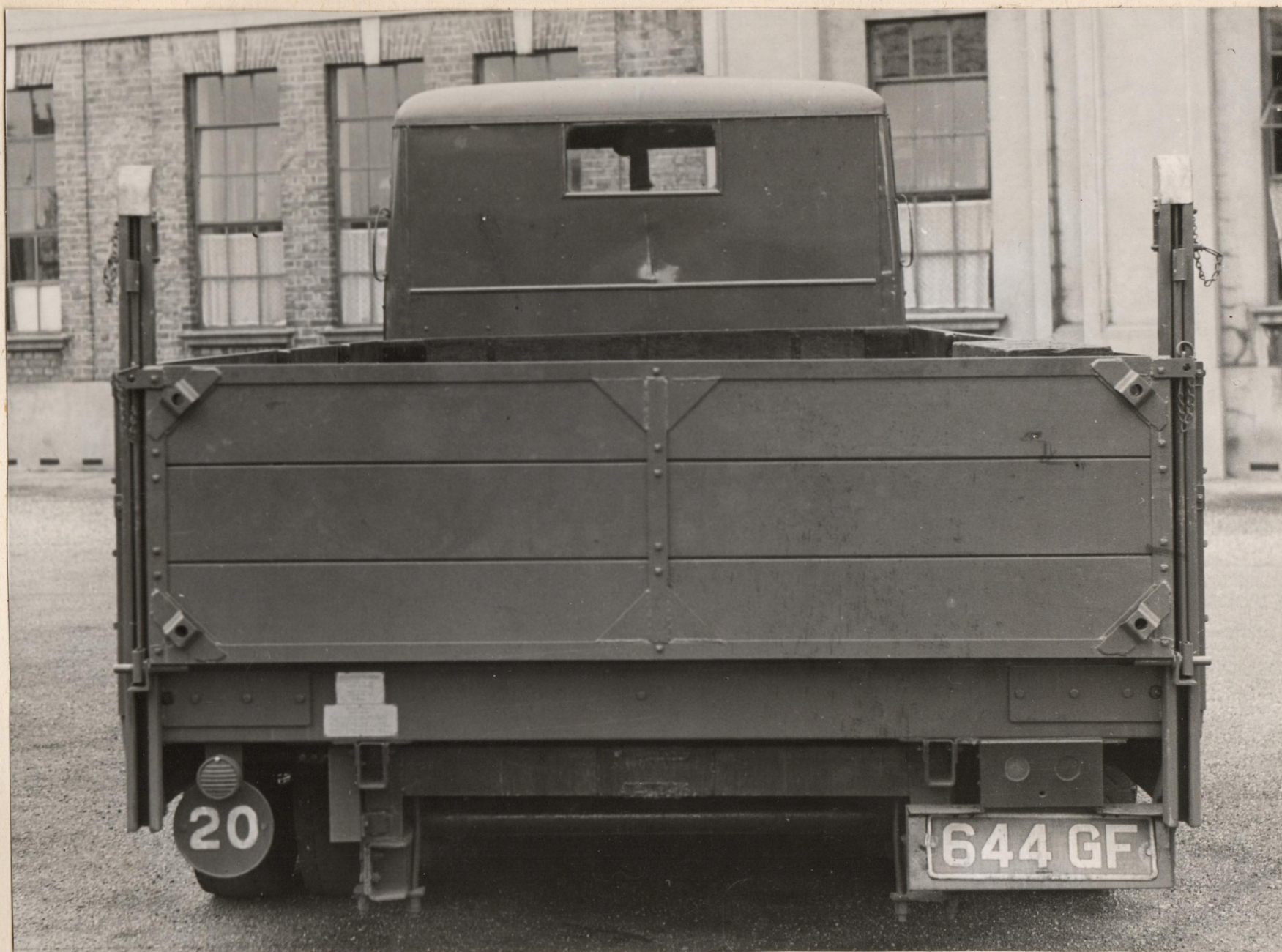
740J - 7 TON BATTERY LORRY WITH BURTONWOOD LOADER TAILBOARD - CLOSED POSITION
