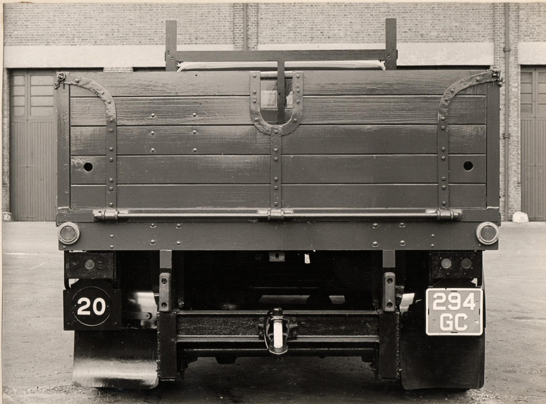
1009J REAR VIEW SHEWING TOWING ATTACHMENT
