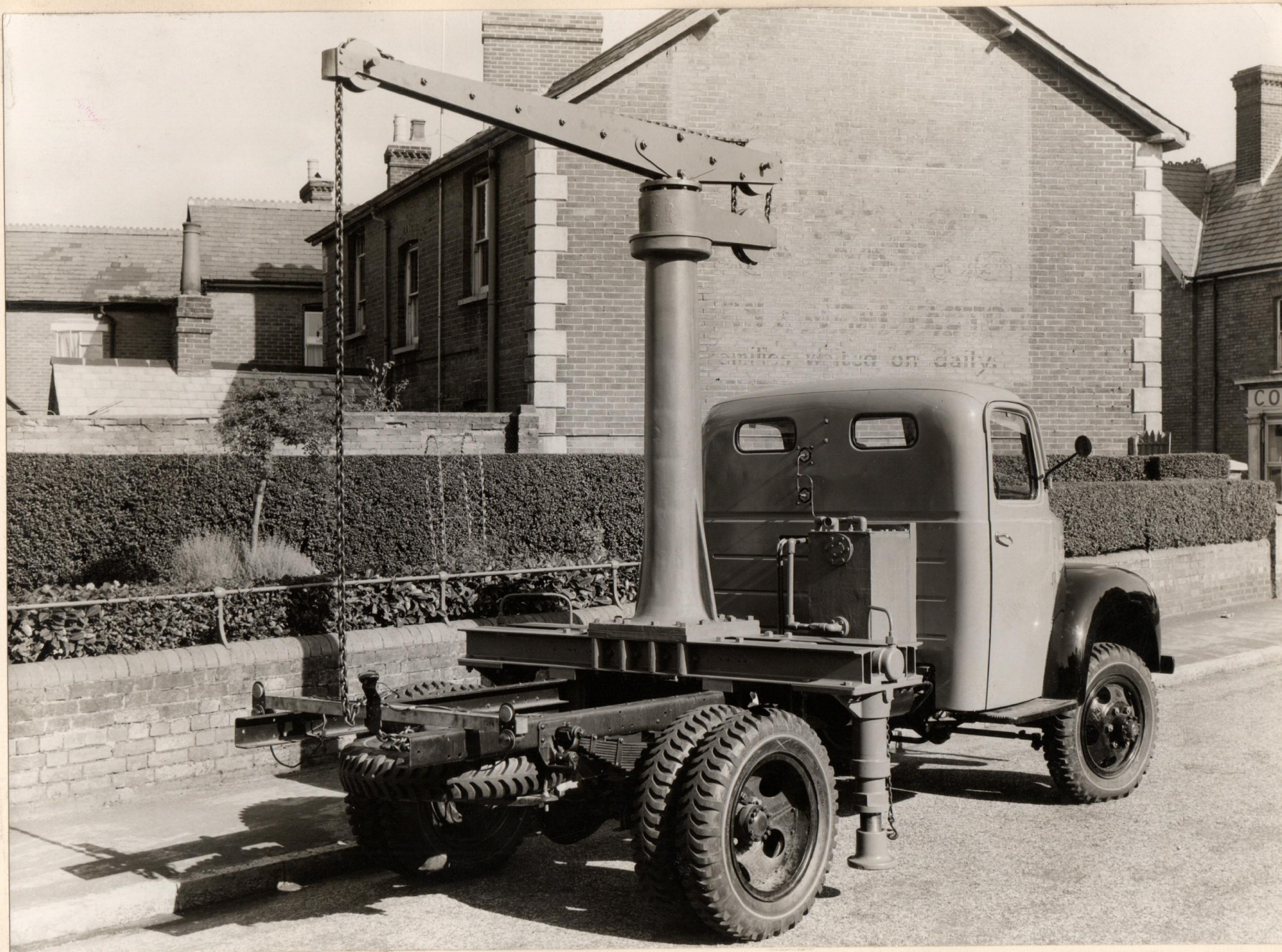
'FLOWERS' 1 TON HYDRAULIC CRANE FITTED TO FORD CHASSIS
