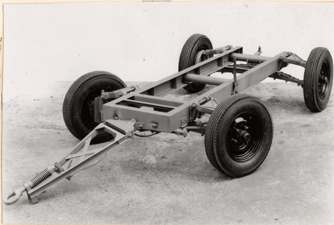
GLOVER WEBB & LIVERSIDGE TRAILER INTERLOCKED DRAWBAR & FRONT AXLE STEERING
