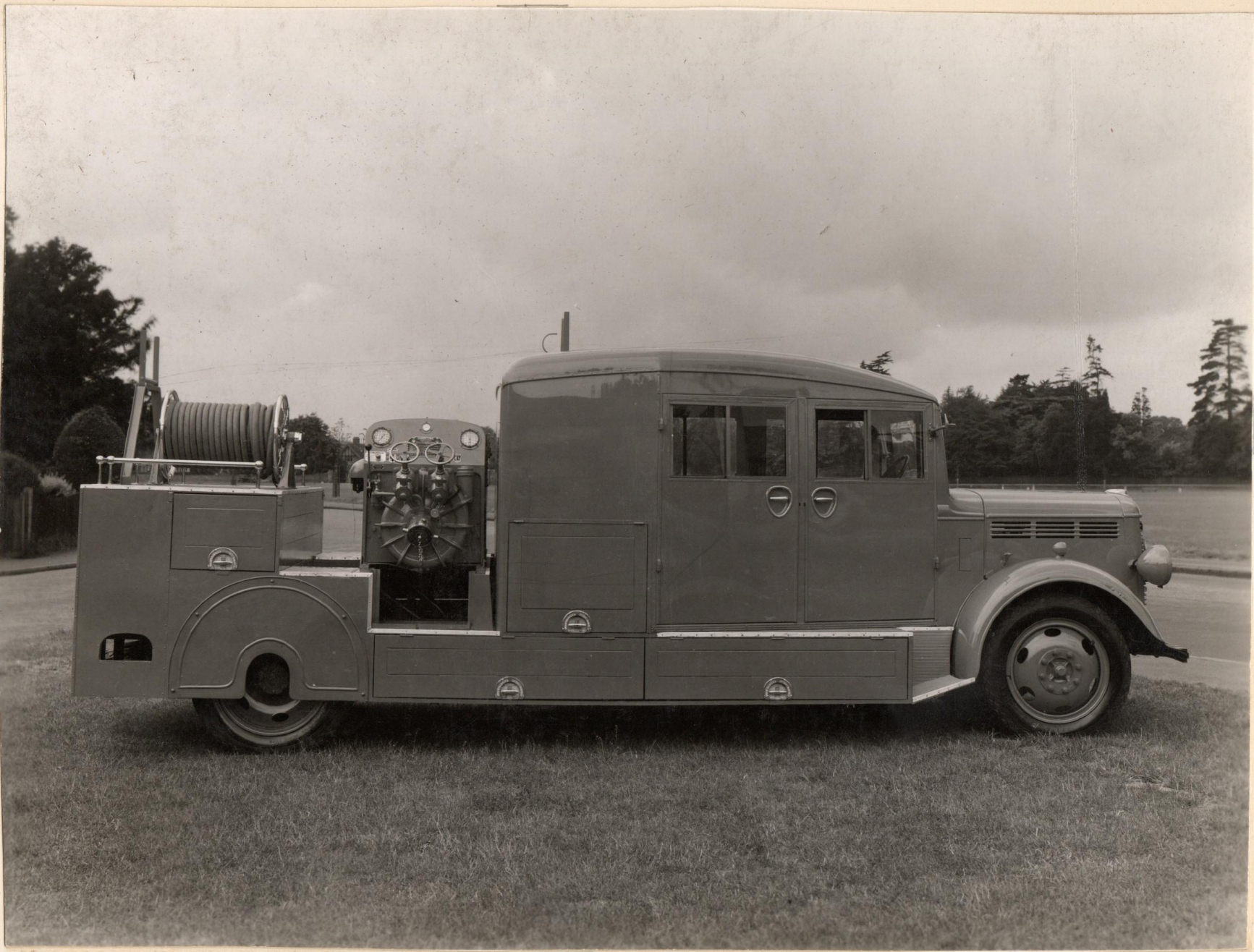
BEDFORD LONG WHEEL BASE FIRE ENGINE O/S VIEW
