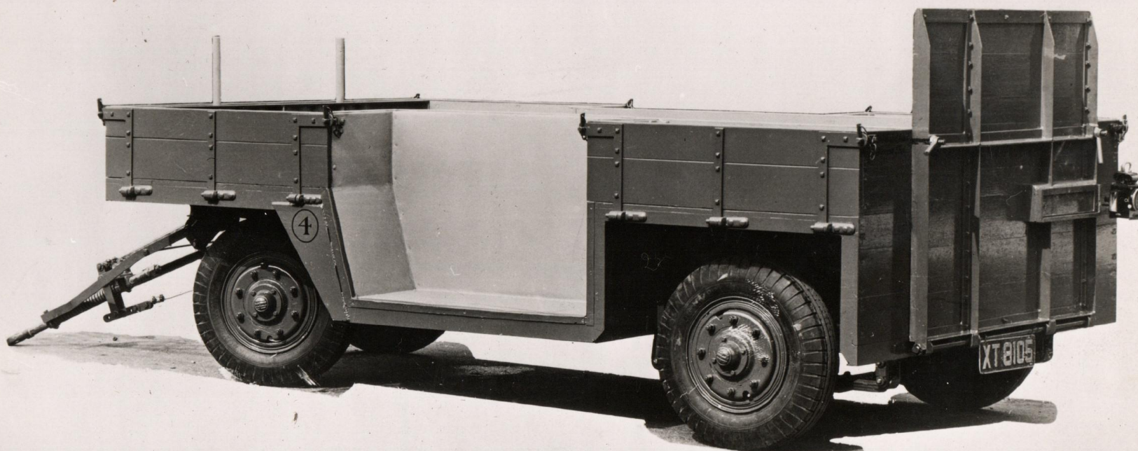
HARROW 2 TON LOW LOADING DROP FRAME TRAILER.
