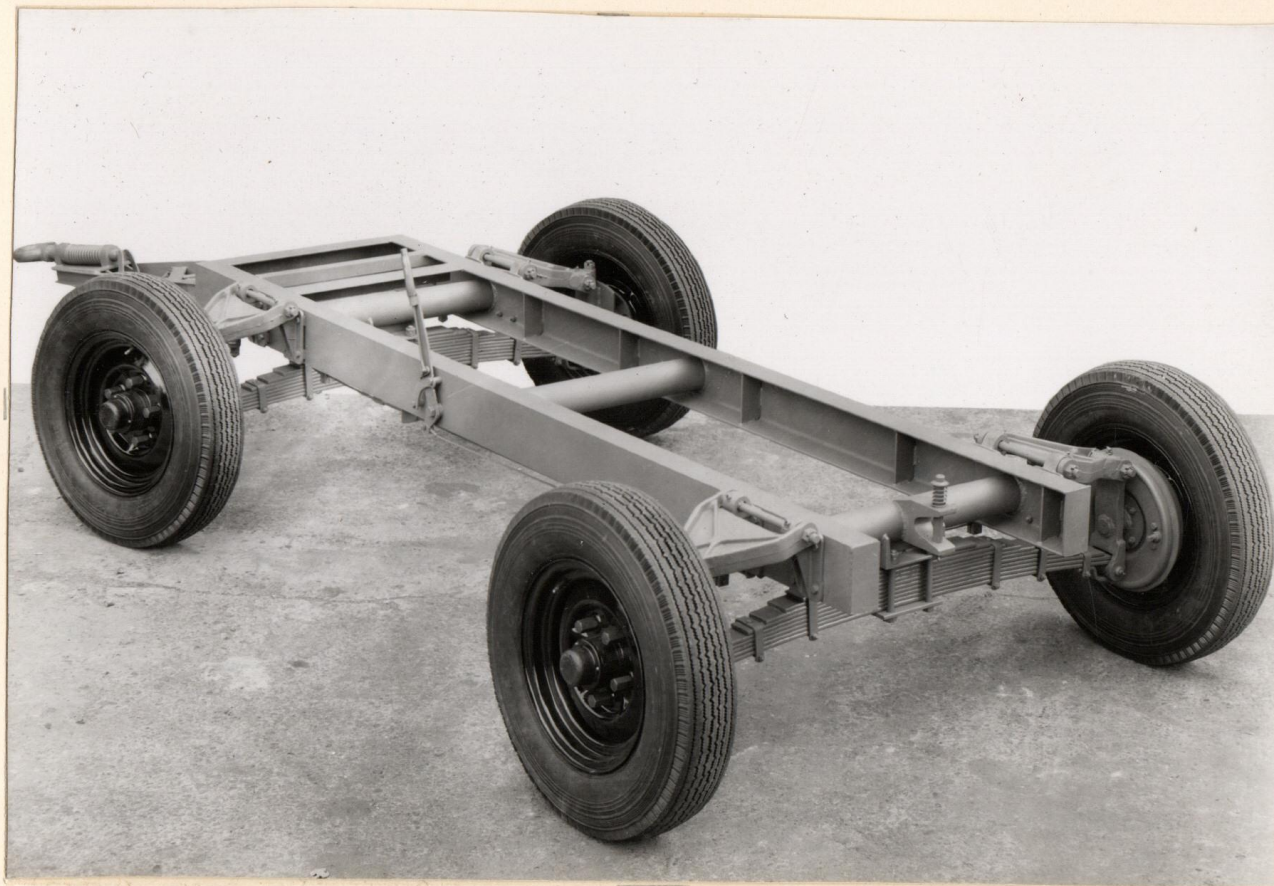
GLOVER WEBB & LIVERSIDGE TRAILER INTERLOCKED DRAWBAR & FRONT AXLE STEERING
