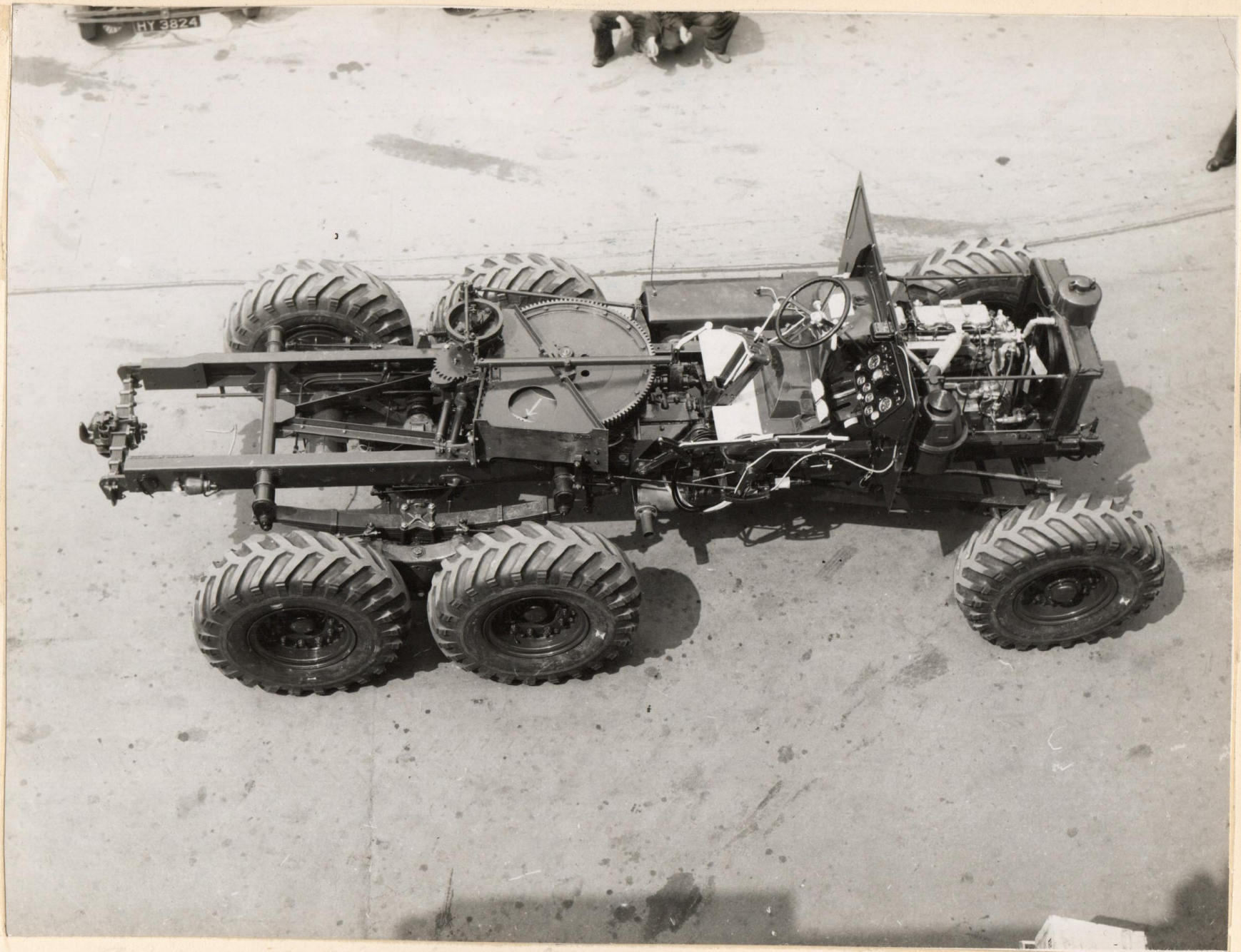
SCAMMELL TRACTOR CHASSIS
